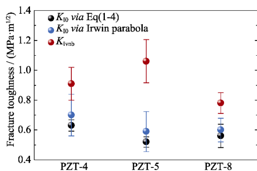
Fig. 4 Fracture toughness K_{Ivnb} and intrinsic fracture toughness K_{I0} for PZT-4, -5, and -8
