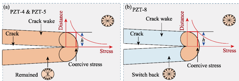
Fig. 5 Illustration of the toughening mechanism (a) PZT-4 and PZT-5; (b) PZT-8
